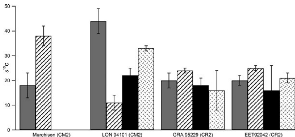
Fig. 5. \delta^{13}\text{C} values for the four-carbon amino acids D- \alpha -ABA (dark gray) and \alpha -AIB (diagonal stripes) and the five-carbon amino acids D-valine (black) and isovaline (checked). Error bars represent standard deviations (see Table 1). There is no clear correlation between the alpha substituent and ^{13}\text{C} enrichment.
