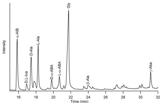
Fig. 1. GC-MS/IRMS chromatogram of the derivatized, acid-hydrolyzed, hot-water extract of EET 92042. The trace shows the m/z 44 ( ^{12}\text{CO}_2 peak) produced and measured during carbon compound-specific isotope analysis. Unidentified peaks represent compounds that could not be adequately identified or analyzed because of coelutions or insufficient sensitivity.
