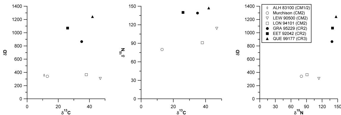
Fig. 6. Isotopic data for glycine in the seven analyzed carbonaceous chondrites. Nitrogen data were not obtained for ALH 83100.
