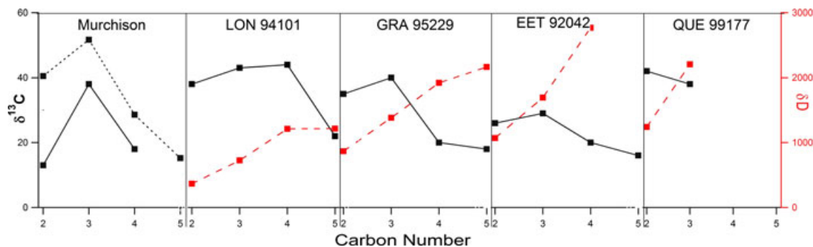
Fig. 3. Carbon and deuterium isotopic data for two- to five-carbon \alpha -amino, \alpha -H amino acids in five carbonaceous chondrites. The black solid line and left axis show the \delta^{13}\text{C} values; the dashed line and right axis show the \delta\text{D} values. The amino acids are: glycine ( \text{C}_2 ), D-alanine ( \text{C}_3 ), D- \alpha -amino- n -butyric acid ( \text{C}_4 ), D-valine ( \text{C}_5 ). The dotted line in the Murchison panel represents data from Pizzarello et al. (2004). No \delta\text{D} data were obtained for the \text{C}_3 , \text{C}_4 , or \text{C}_5 \alpha -amino, \alpha -H amino acids in Murchison.
