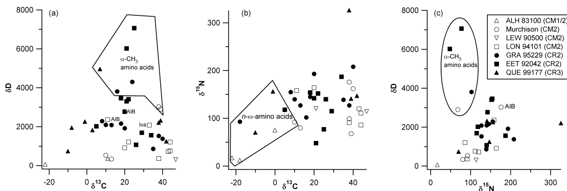
Fig. 2. Isotopic data for the amino acids in the seven analyzed carbonaceous chondrites. Outlined areas highlight subsets of structurally similar compounds.
