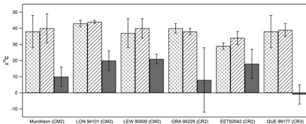
Fig. 4. \delta^{13}\text{C} values for D-alanine (checked), L-alanine (striped), and \beta -alanine (solid) in six carbonaceous chondrites. Error bars represent standard deviations (see Table 1). \beta -Alanine is consistently less enriched in ^{13}\text{C} , perhaps reflecting a different formation pathway.
