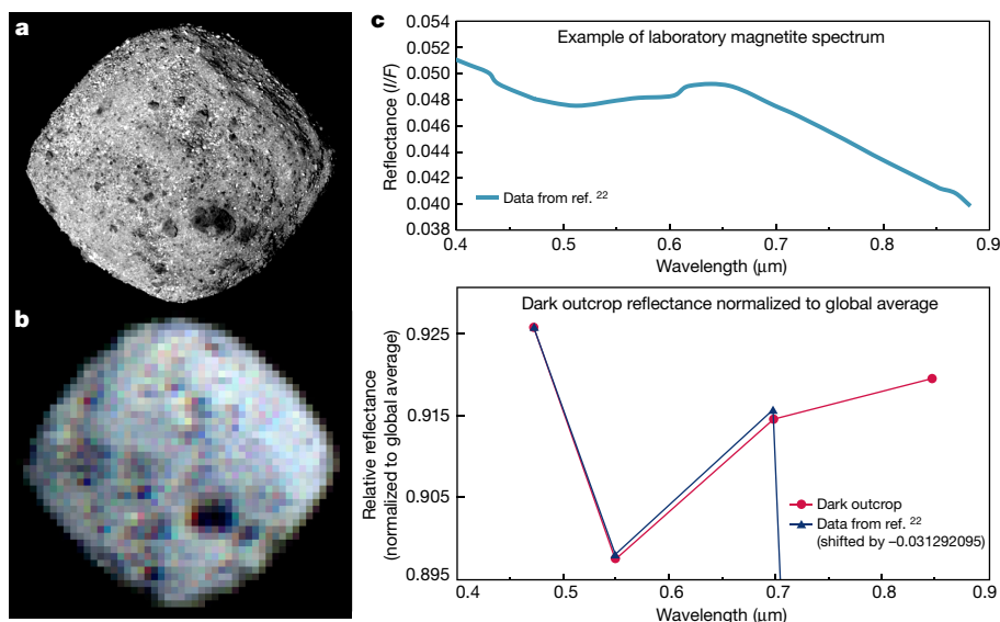
Fig. 2 | OCAMS imaging data elucidate Bennu's diverse surface reflectance and composition. a , Image acquired by the PolyCam imager on 25 November 2018 at a phase angle of about 5° and a pixel scale of about 1.1 m per pixel. b , Colour mosaic acquired by the MapCam imager 9 on 8 November 2018 at a phase angle of about 5° and a pixel scale of 10.9 m per pixel (coarse pixel scale is due to the wider field of view of MapCam at the larger observing distance). c , The upper plot shows a
