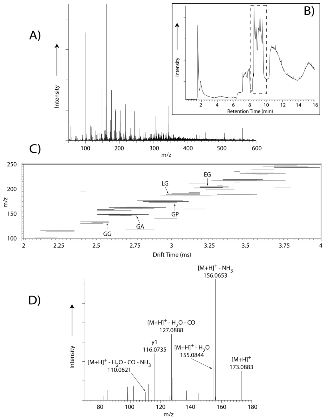
Figure S1. UPLC-Q-TWIMS-TOF-MS data demonstrating how dipeptides were identified in the archived cyanamide samples. Data from fraction 57-67 are shown here as an example. A) An averaged mass spectrum for the 8-10 minute region of the UPLC total ion chromatogram (B), exhibiting the vast chemical complexity of the samples studied here. C) TWIMS-TOF-MS m/z vs drift time plot for the 8-10 minute region of (B), where a suite of glycine-containing dipeptides are separated based on specific drift times. D) Following TWIMS separation, MS/MS spectra were obtained to confirm dipeptide detection by the presence of the [M+H]^+ ion, along with its corresponding fragment ions produced by collisional dissociation in the transfer cell; shown here is the MS/MS spectrum for glycyproline. Here, GG = glycyglycine, GA = glycyalalanine, GP = glycyproline, LG = leucylglycine, EG = glutamylglycine.
