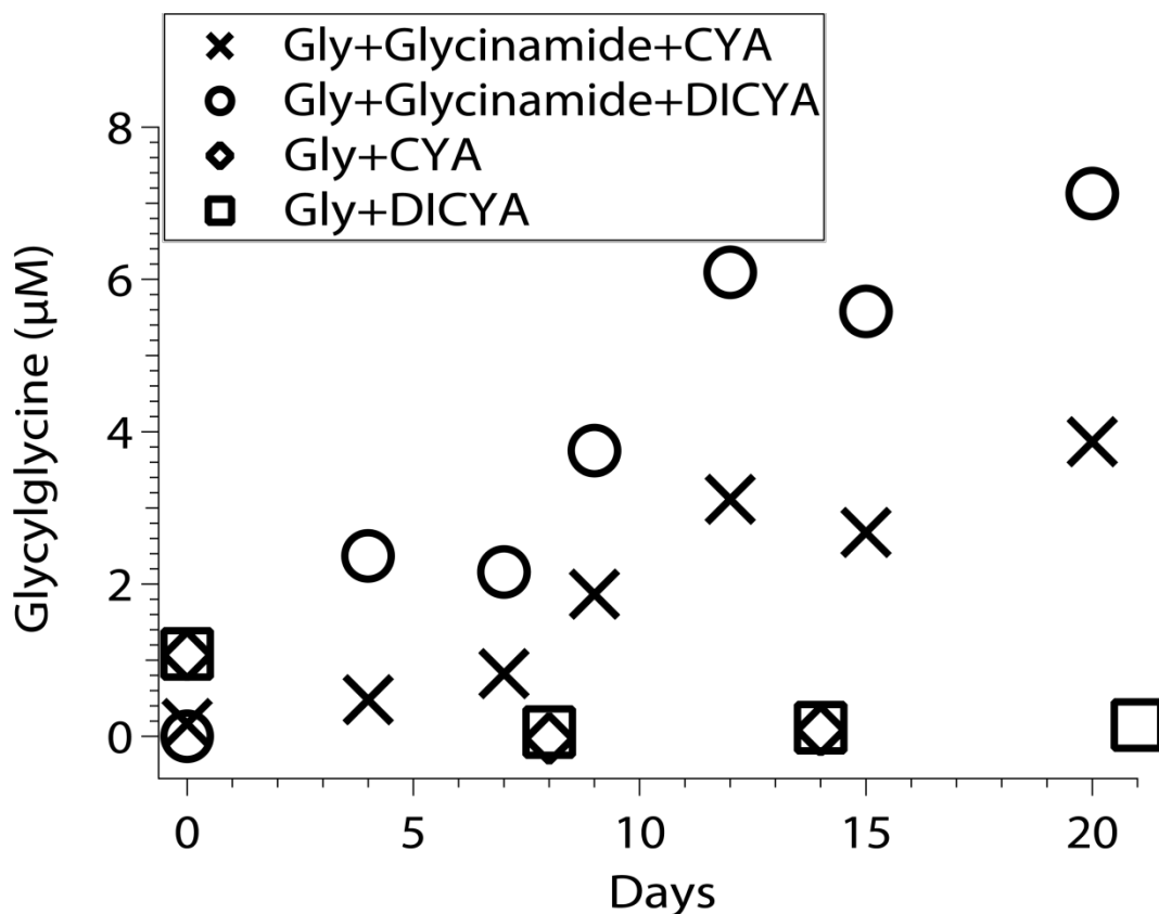
Figure S3. Change in glycyglycine concentration over time as observed from the analysis of heating experiment samples that contained glycine, and cyanamide (CYA) or dicyandiamide (DICYA), as well as glycine, glycineamide, and CYA or DICYA, in a basic solution. The pH values of the solutions shown here are as follows: Gly + CYA = 9.15, Gly + DICYA = 9.18, Gly + Glycinamide + CYA = 8.85, Gly + Glycinamide + DICYA = 8.42.
