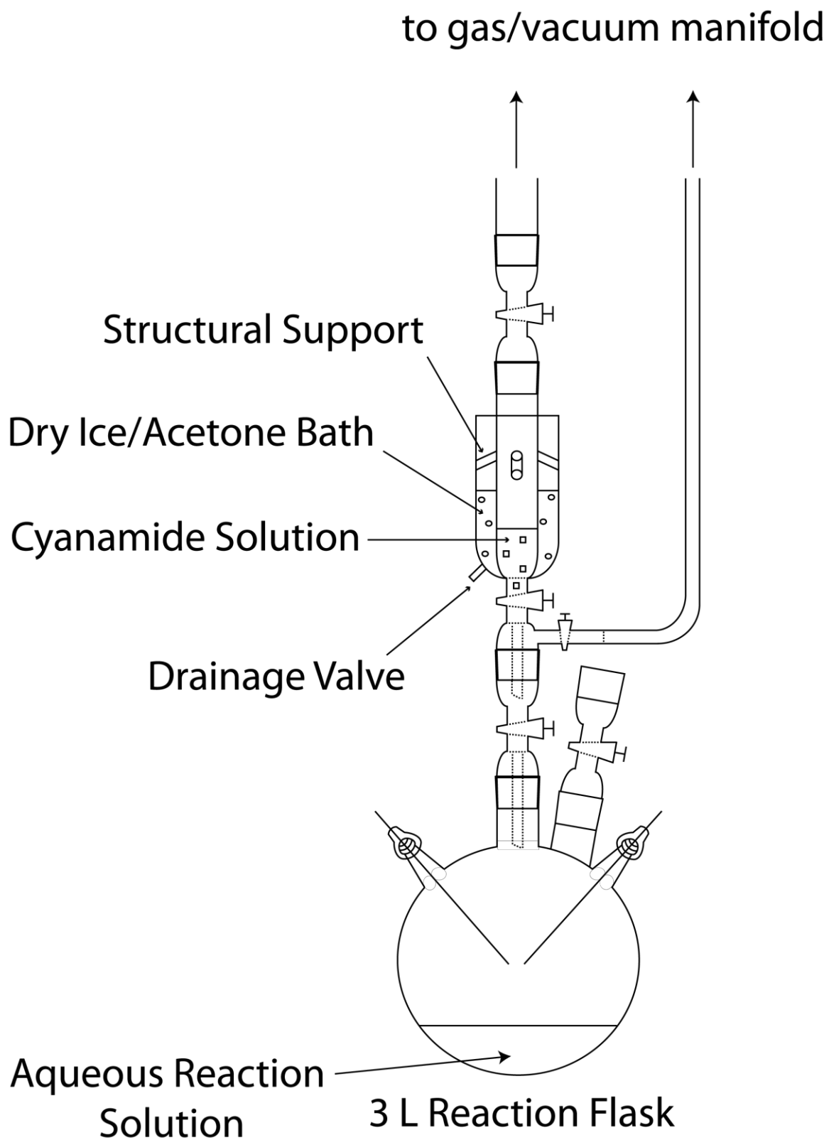
Figure S2. Schematic diagram of the setup used to conduct aqueous cyanamide introductions into the reaction apparatus without compromising the seal of, or introducing contaminants into, the flask while repeating Miller's cyanamide spark discharge experiment.
