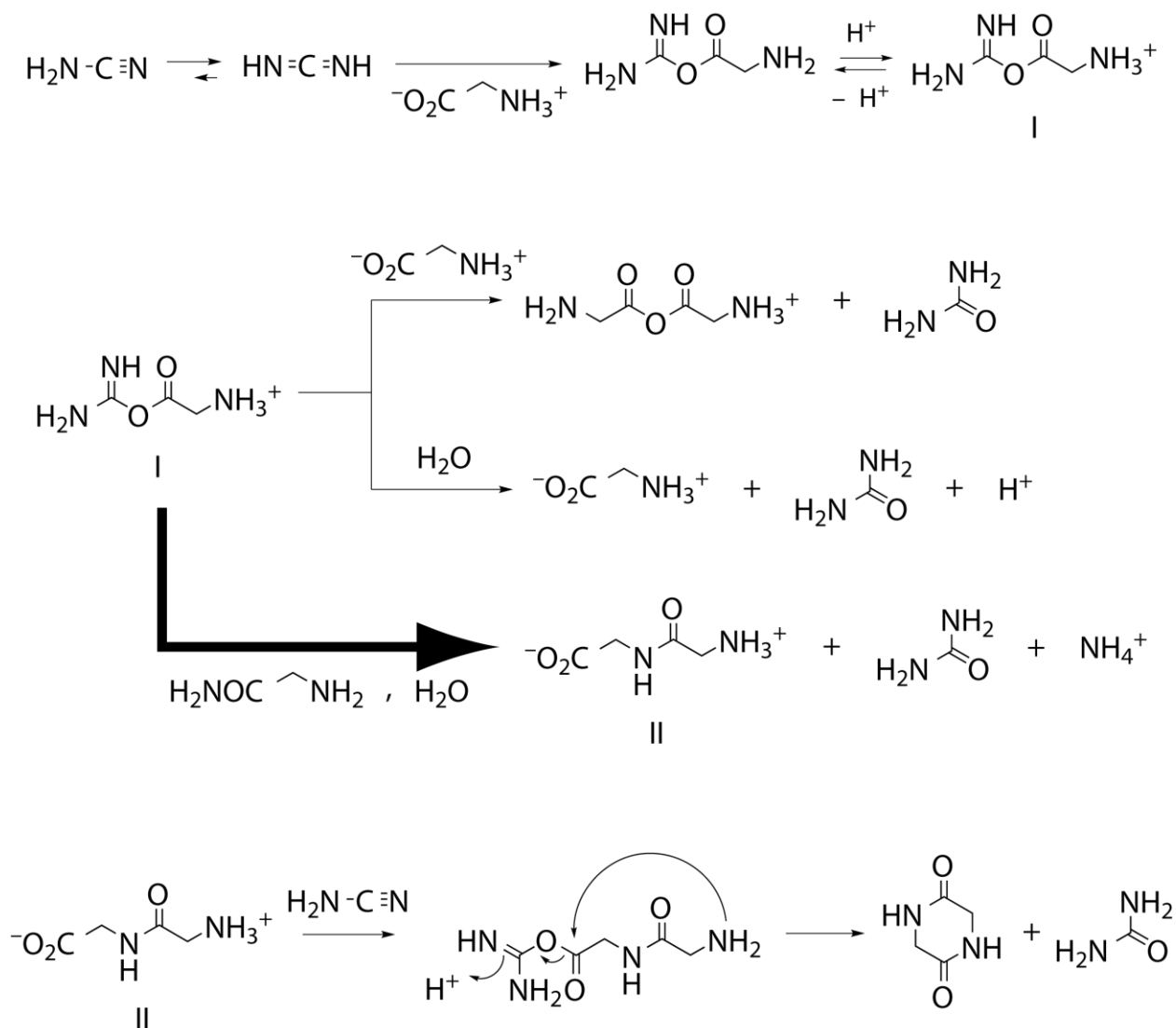
Figure S4. Scheme showing cyanamide-mediated amino acid polymerization reactions. Cyanamide reacts with an amino acid, glycine is shown as an example, to form an activated monomer (I). Once (I) is formed, it can undergo reaction with glycine to yield glycine anhydride, or with water to produce the original amino acid, among other by-products. The \text{pK}_a of the amino group in the amide, glycylglycine is shown here as an example, is \sim 8 at pH values > \sim 8 , [S16] therefore the reaction of (I) with the amide is the favored reaction (bolded arrow) within a basic chemical environment to form the linear dipeptide (II). Product (II) can then react directly with cyanamide to undergo ring formation to yield the DKP. The scheme portrayed here is based in part on previously reported literature. [S15]
